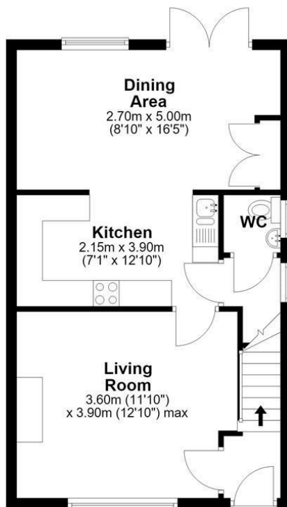
Ground Floor Approx. 43.2 sq. metres (464.8 sq. feet)
