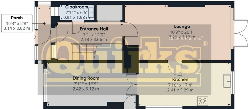
Floor 0
